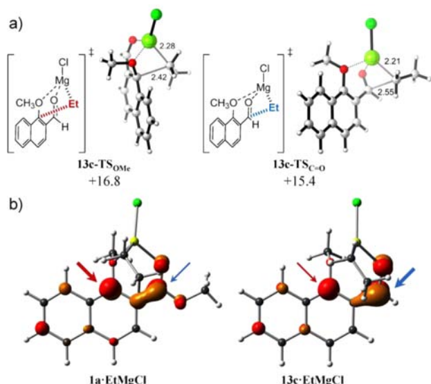
Figure 7. (a) Lowest-energy transition structures and activation free energies ( \Delta G^\ddagger ) for the reaction of naphthyl aldehyde 13c and \text{EtMgCl} calculated at the PCM(THF)/B3LYP/6-31G(d) level. Energies are in \text{kcal mol}^{-1} and distances are in Angstroms. (b) Isosurface representation of LUMO of reactant complex derived from ester 1a and aldehyde 13c . Potentially reactive positions are marked with red (methoxy group) and blue (carbonyl group) arrows.
