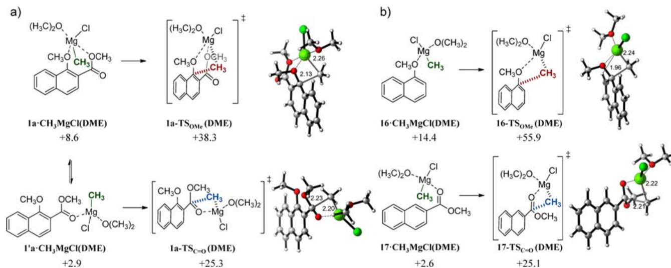
Figure 8. (a) Lowest-energy reactant complexes and transition structures for the reaction of naphthyl ester 1a and \text{CH}_3\text{MgCl}(\text{DME}) . (b) Lowest-energy reactant complexes and transition structures for the reaction of 1-methoxynaphthalene 16 and methyl 2-naphthoate 17 with \text{CH}_3\text{MgCl}(\text{DME}) . Complexation ( \Delta G ) and activation free energies ( \Delta G^\ddagger ) were calculated at the PCM(THF)/B3LYP/6-31G(d) level and are related to the isolated reactants. Energies are in \text{kcal mol}^{-1} and distances are in Angstroms.
