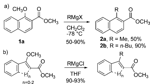
Scheme 1. Displacement of Alkoxy Groups by Grignard Reagents in (a) Aromatic and (b) Nonaromatic Substrates
