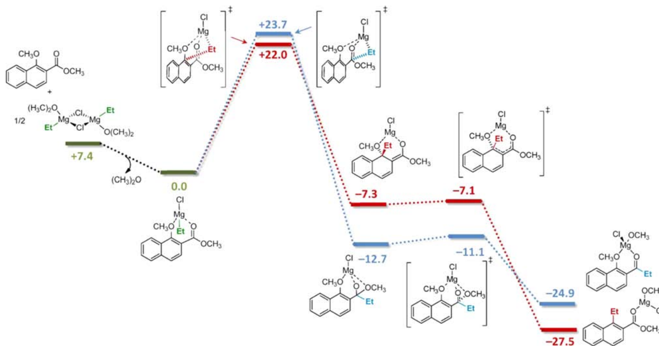
Figure 3. Reaction pathways for the addition of Grignard reagents to aromatic 1,2-alkoxy esters calculated at the PCM(THF)/B3LYP/6-31G(d) level. Free energies ( \Delta G ) relative to the reactant complex are in kcal mol -1 .
