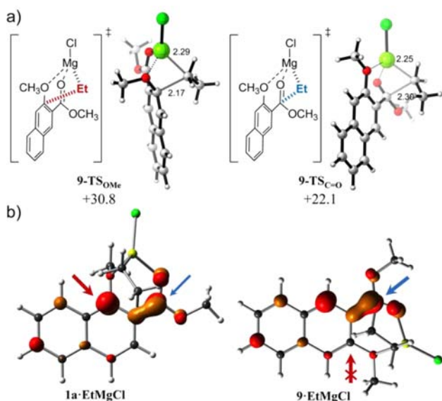
Figure 4. (a) Lowest-energy transition structures and activation free energies ( \Delta G^\ddagger ) for the reaction of naphthyl ester 9 and EtMgCl calculated at the PCM(THF)/B3LYP/6-31G(d) level. Energies are in kcal mol -1 and distances are in Angstroms. (b) Isosurface representation of LUMO of reactant complexes of isomers 1a and 9 . Potentially reactive positions are marked with red (methoxy group) and blue (carbonyl group) arrows.
