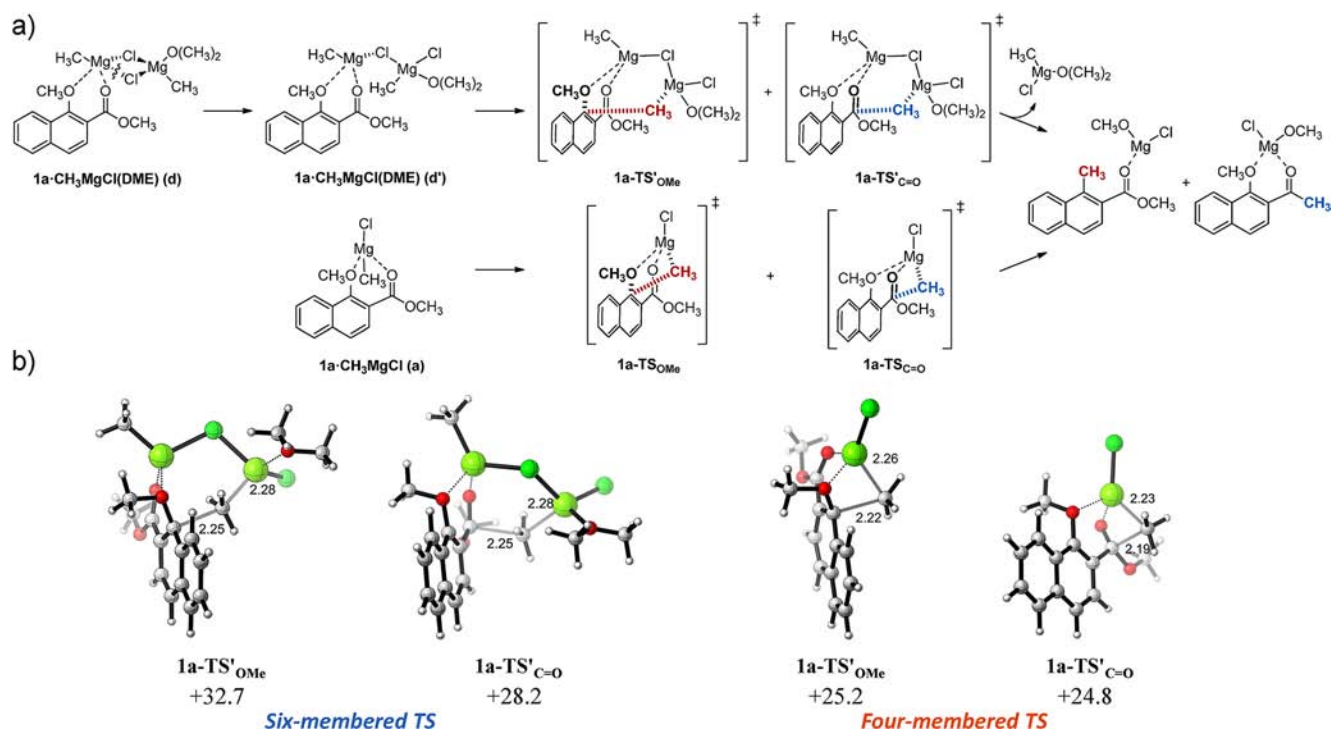
Figure 2. (a) Proposed mechanisms for the reaction of vinyllogous 1,2-alkoxy carbonyl compounds with Grignard reagents through six-membered (TS') and four-membered (TS) cyclic transition states. (b) Most relevant transition structures and activation free energies ( \Delta G^\ddagger ) calculated at the PCM(THF)/B3LYP/6-31G(d) level. Energies are in kcal mol -1 and distances are in Angstroms.
