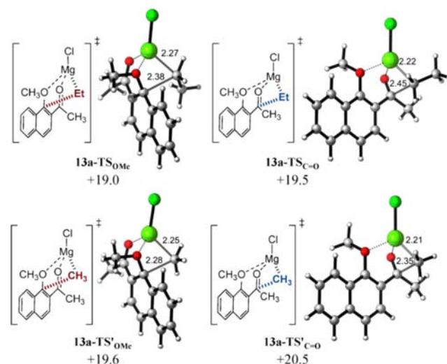
Figure 6. Lowest-energy transition structures and activation free energies ( \Delta G^\ddagger ) for the reaction of naphthyl ketone 13a with EtMgCl (top) and MeMgCl (bottom) calculated at the PCM(THF)/B3LYP/6-31G(d) level. Energies are in kcal mol -1 and distances are in Angstroms.
