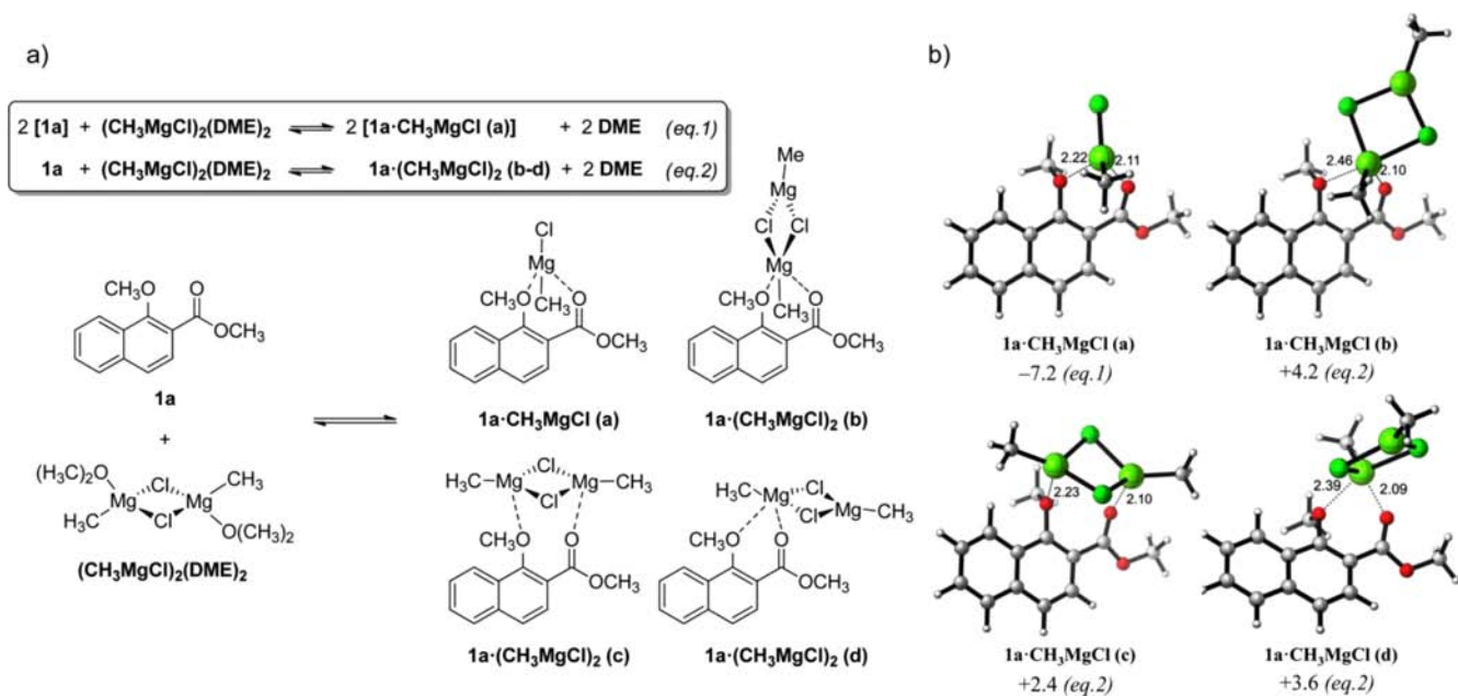
Figure 1. (a) Proposed coordination of Grignard reagents to vinyllogous 1,2-alkoxy carbonyl compounds leading to 1:1 and 2:1 complexes (eq. 1 and eq. 2, respectively). Additional coordination modes are described in the Supporting Information. (b) Structures and complexation free energies ( \Delta G_{\text{complex}} ) calculated at the PCM(THF)/B3LYP/6-31G(d) level. Energies are in kcal mol -1 and distances are in Angstroms.
