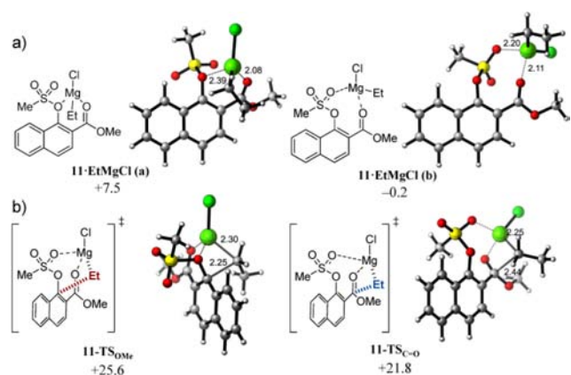
Figure 5. (a) Six-membered (left) and eight-membered (right) chelate reactant complexes of (mesyl)naphthyl ester 11 with EtMgCl together with their respective complexation free energies ( \Delta G_{\text{complex}} ). (b) Lowest-energy transition structures and activation free energies ( \Delta G^\ddagger ) for the reaction of 11 and EtMgCl calculated at the PCM(CH 2 Cl 2 )/B3LYP/6-31G(d) level. Energies are in kcal mol -1 and distances are in Angstroms.
